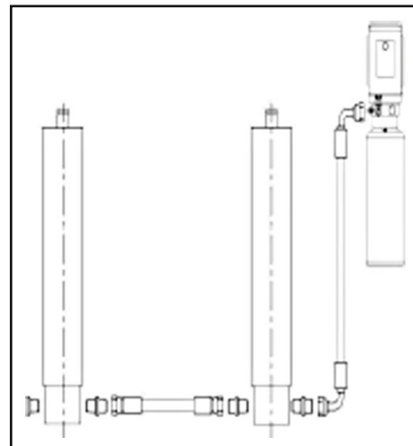
Figure 10 Connexions hydrauliques
